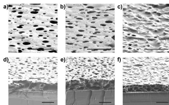
Figure 4. Surface and cross-sectional SEM images of PFS-VImTf 2 N/PAA complex membrane: untreated membrane (a and d), after oxidation by 10 mM Fe(ClO 4 ) 3 aqueous solution (b and e), and then following reduction by 10 mM ascorbic acid in aqueous solution (c and f). Scale bar: 1 μm.
